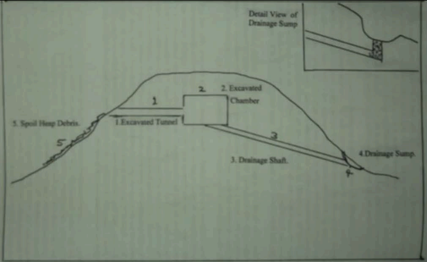
Elevation View of Tunnel, Chamber and Drains.
